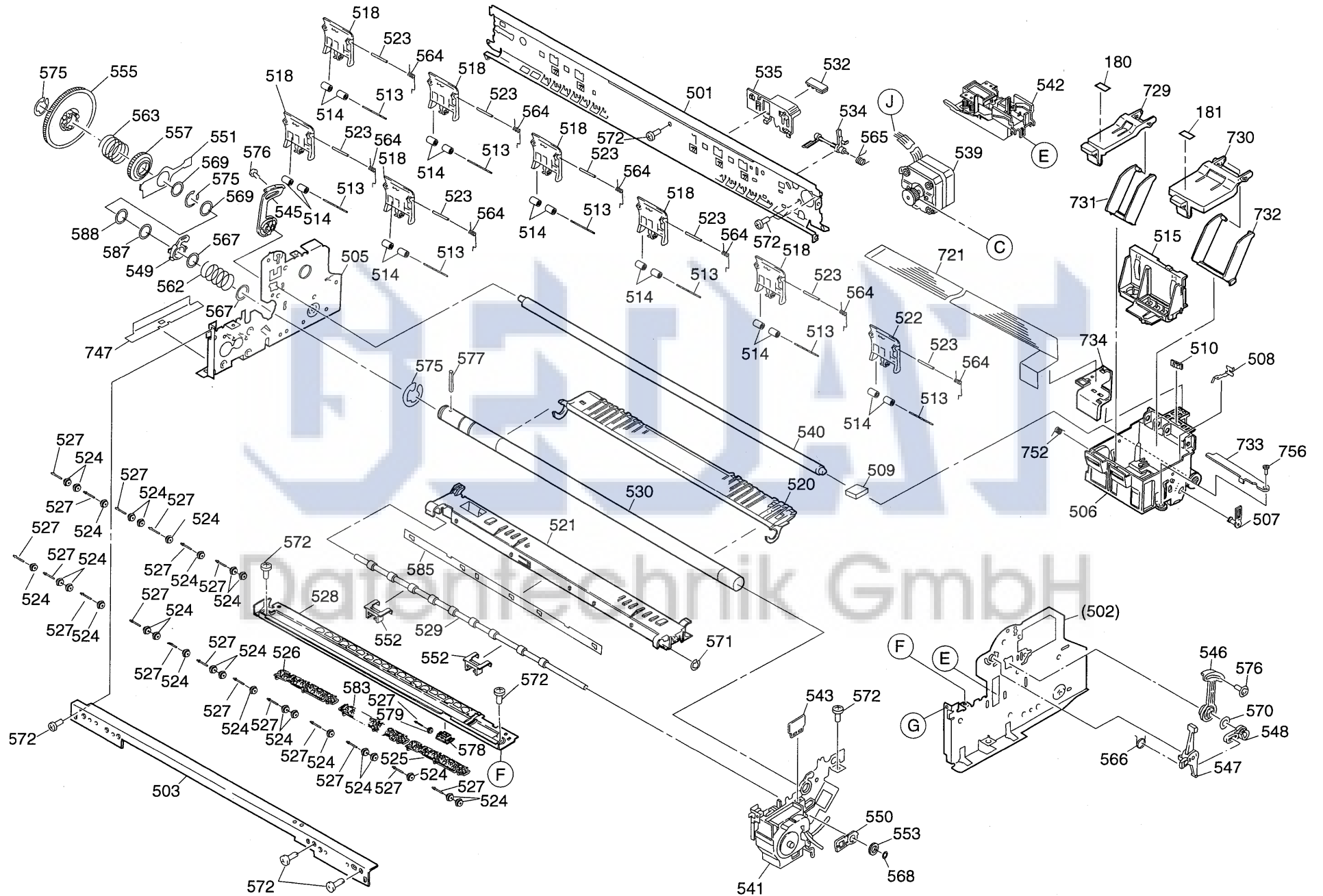
EXPLODED DIAGRAM FOR EPSON STYLUS Photo EX / PM-2000C (3/3)
