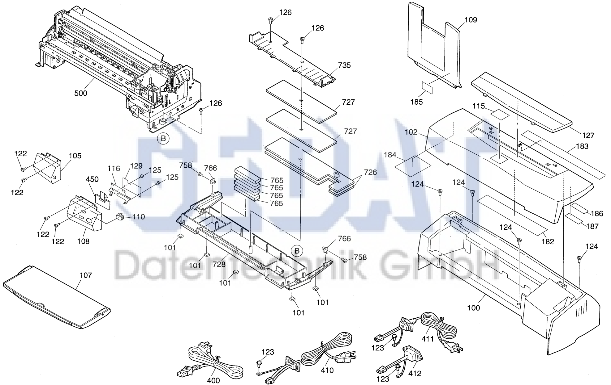
EXPLODED DIAGRAM FOR EPSON STYLUS Photo EX / PM-2000C (1/3)
