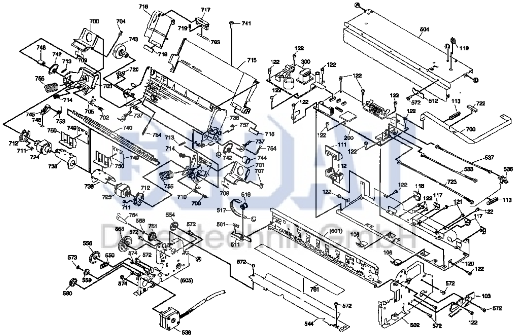
EXPLODED DIAGRAM FOR EPSON STYLUS Photo 700
