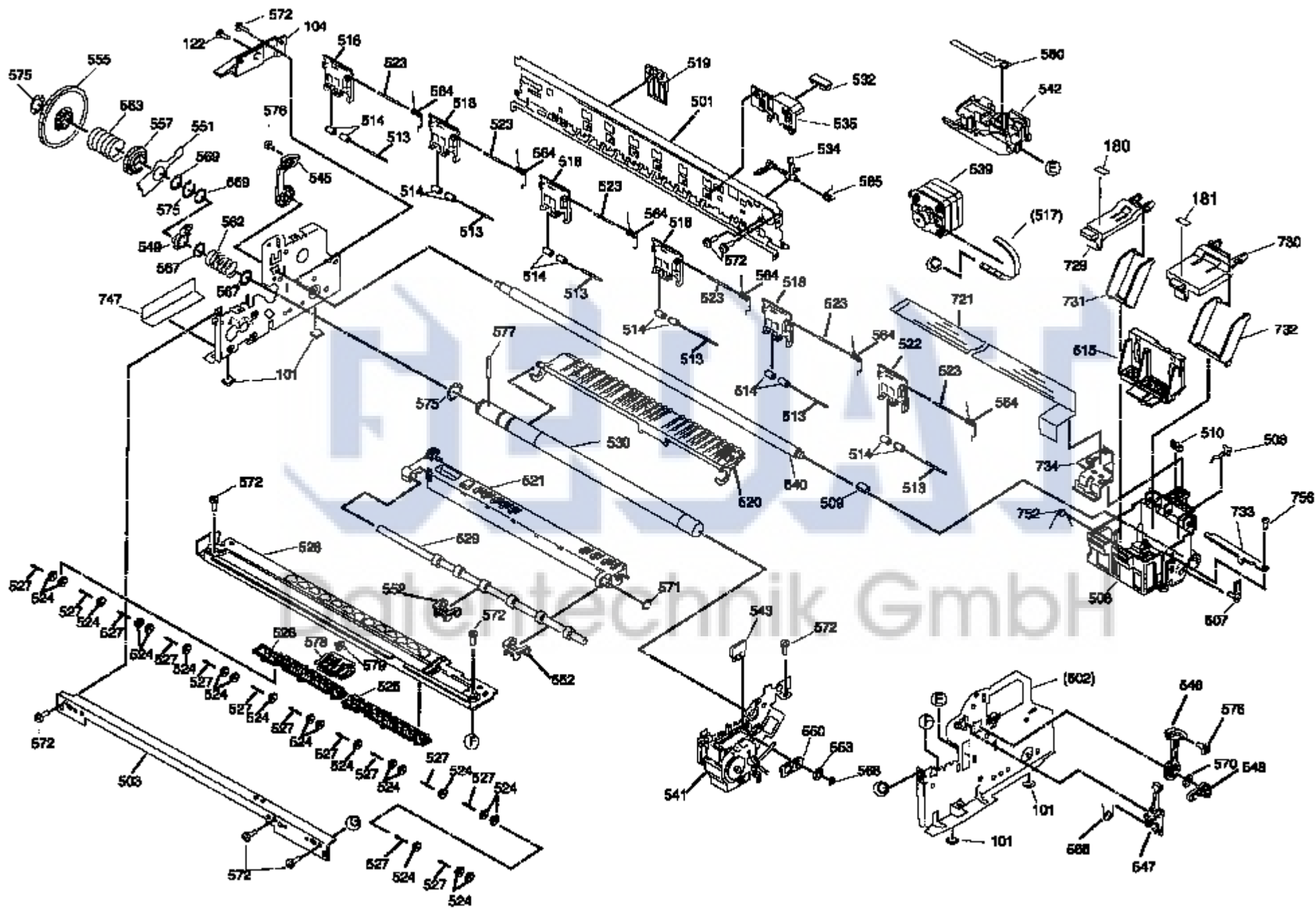
EXPLODED DIAGRAM FOR EPSON STYLUS Photo 700
